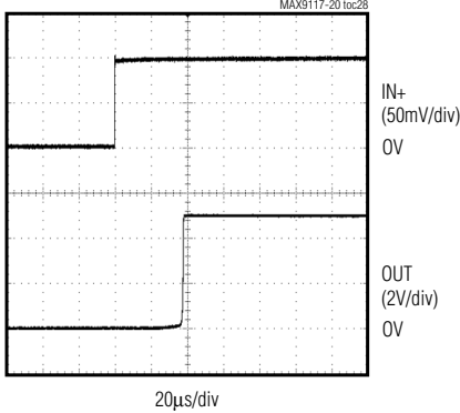
MAX9117/MAX9119 PROPAGATION DELAY ( t_{PD+} ) ( V_{CC} = +5V )
